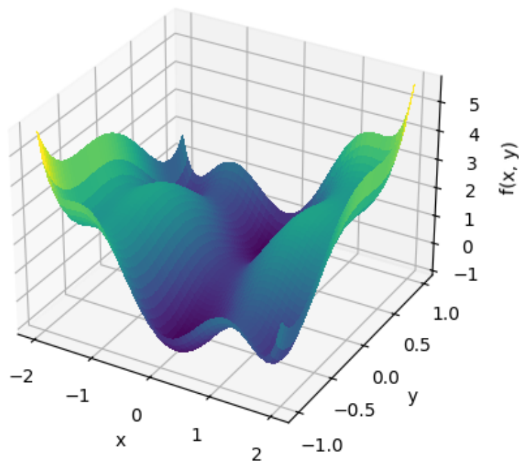
Six-hump Camelback function
